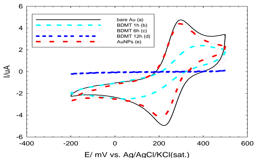
Figure 4. The CVs obtained at a scan rate of 150 \text{ mVs}^{-1} for 1\text{mM K}_3[\text{Fe}(\text{CN})_6] in 0.1\text{M KCl} at (a) bare Au electrode, (b,c,d) BDMT/Au electrodes (diameter=1.6 mm) prepared by soaking the poly-Au electrode in BDMT solution for 1,6, and 12 h respectively.
