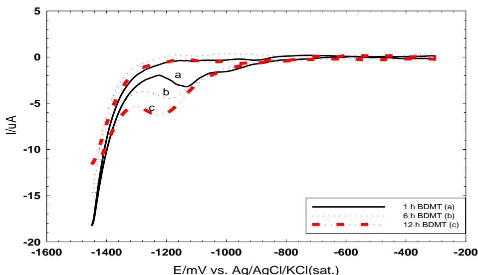
Figure 3. The CVs for the reductive desorption of BDMT self-assembled for 1 (a), 6 (b), and 12 (c) h on poly- Au electrode measured in 0.5 M KOH solution. Potential scan rate: 50 mVs -1 .
