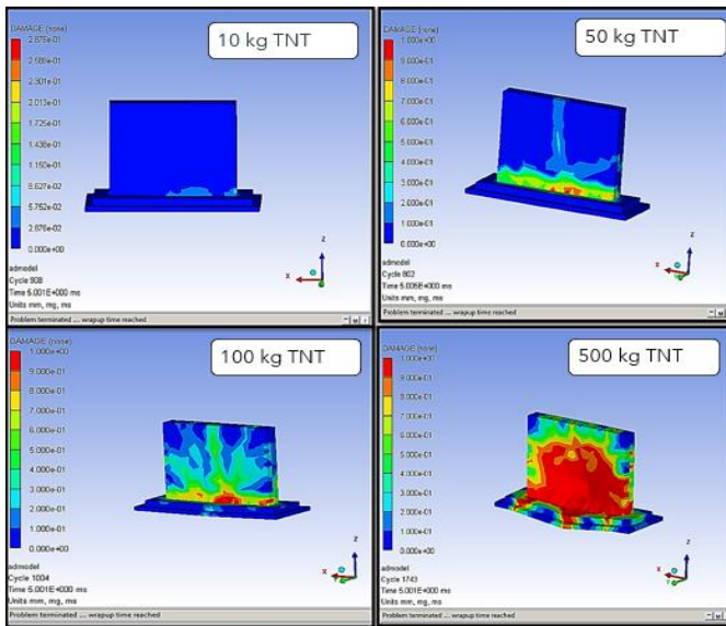
Fig. 11. Damage simulations
