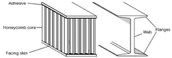
Fig. 3. Mechanical similarities between sandwich panel and I beam.
