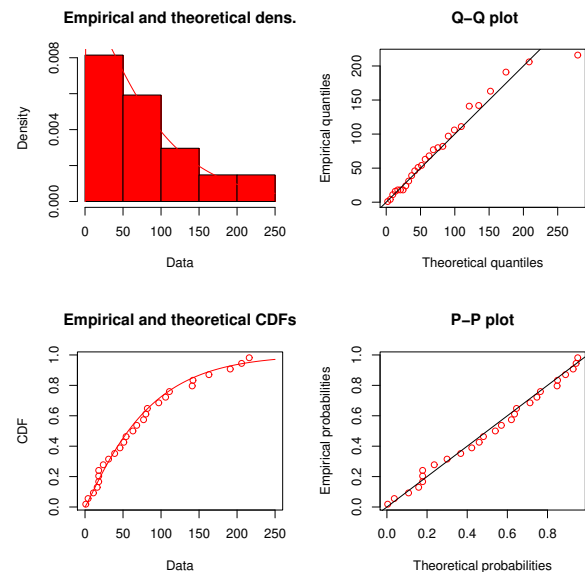
Fig. 7: Fitted second sample
