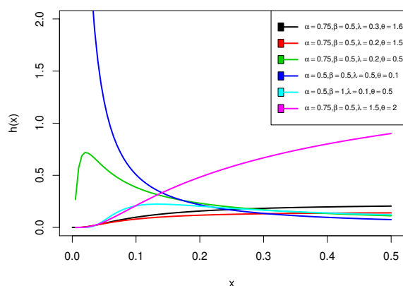
Fig. 4: Hazard rate function for WFr model
