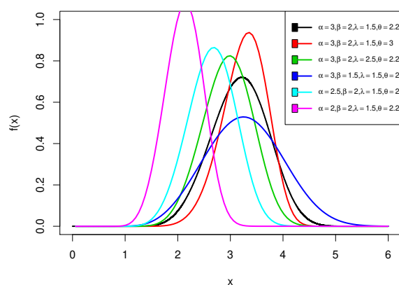
Fig. 1: pdf for WFr model
