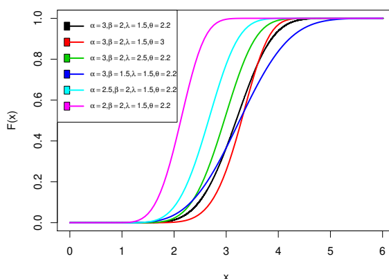
Fig. 2: cdf for WFr model
