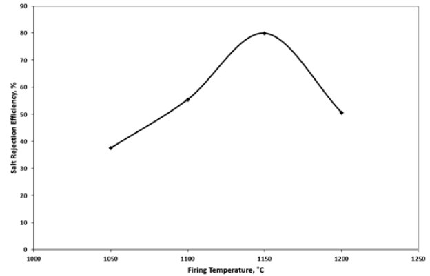
Fig. 8: Salt Rejection for Support Ceramic Membranes
