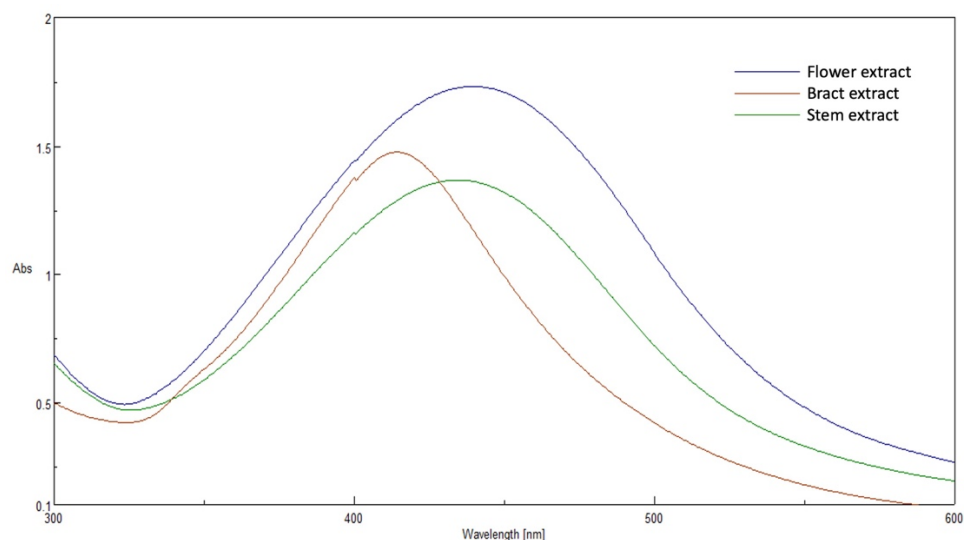
Figure 1. The UV-visible spectrum of prepared AgNPs using extracts of different parts of Cynara scolymus .
